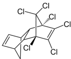
Figure 1: Structural formula of aldrin
