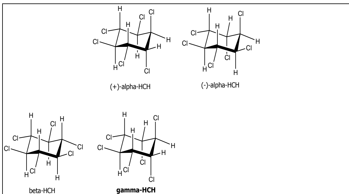
Figure 9: Structural formulas of lindane (gamma-HCH), alpha-HCH and beta-HCH
