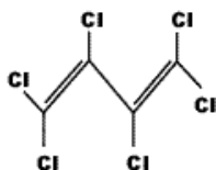
Figure 8: Structural formula of hexachlorobutadiene
