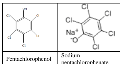
Figure 12: Structural formulas of PCP and its sodium salt
