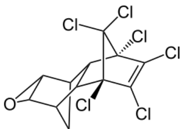
Figure 4: Structural formula of dieldrin
