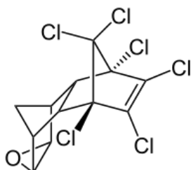
Figure 5: Structural formula of endrin
