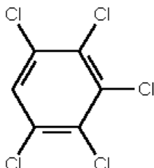
Figure 11: Structural formula of pentachlorobenzene
