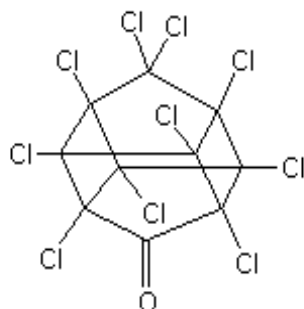
Figure 3: Structural formula of chlordecone
