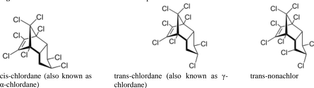
Figure 2: Structural formulas of chlordane components
