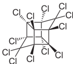
Figure 10: Structural formula of mirex
