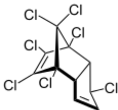
Figure 6: Structural formula of heptachlor
