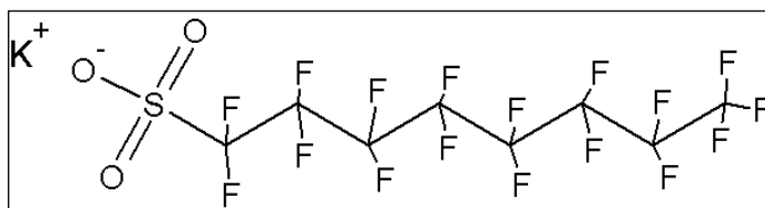
Figure 13: Structural formula of PFOS
