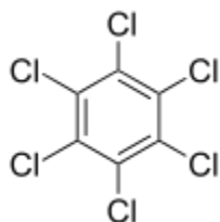
Figure 7: Structural formula of hexachlorobezene
